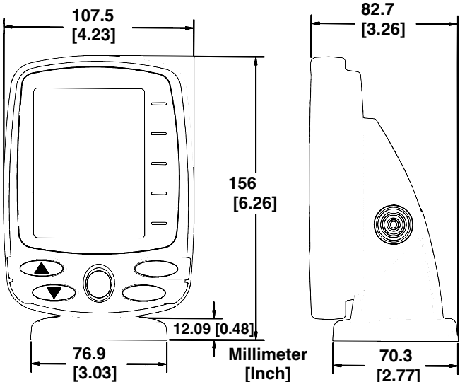
Front view (left) and side view (right) showing dimensions of the X67C when mounted on quick release bracket.
