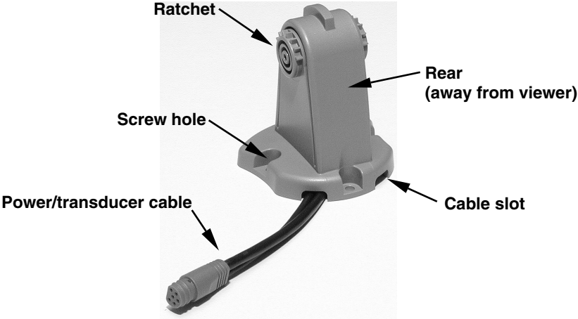
X67C quick release mounting bracket. Slots in the base allow routing the cable from beneath the mount.
