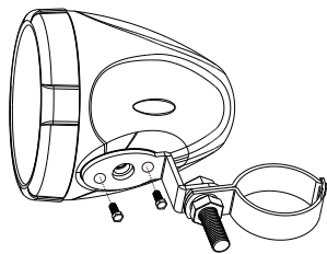
Loudspeaker mounting diagram
